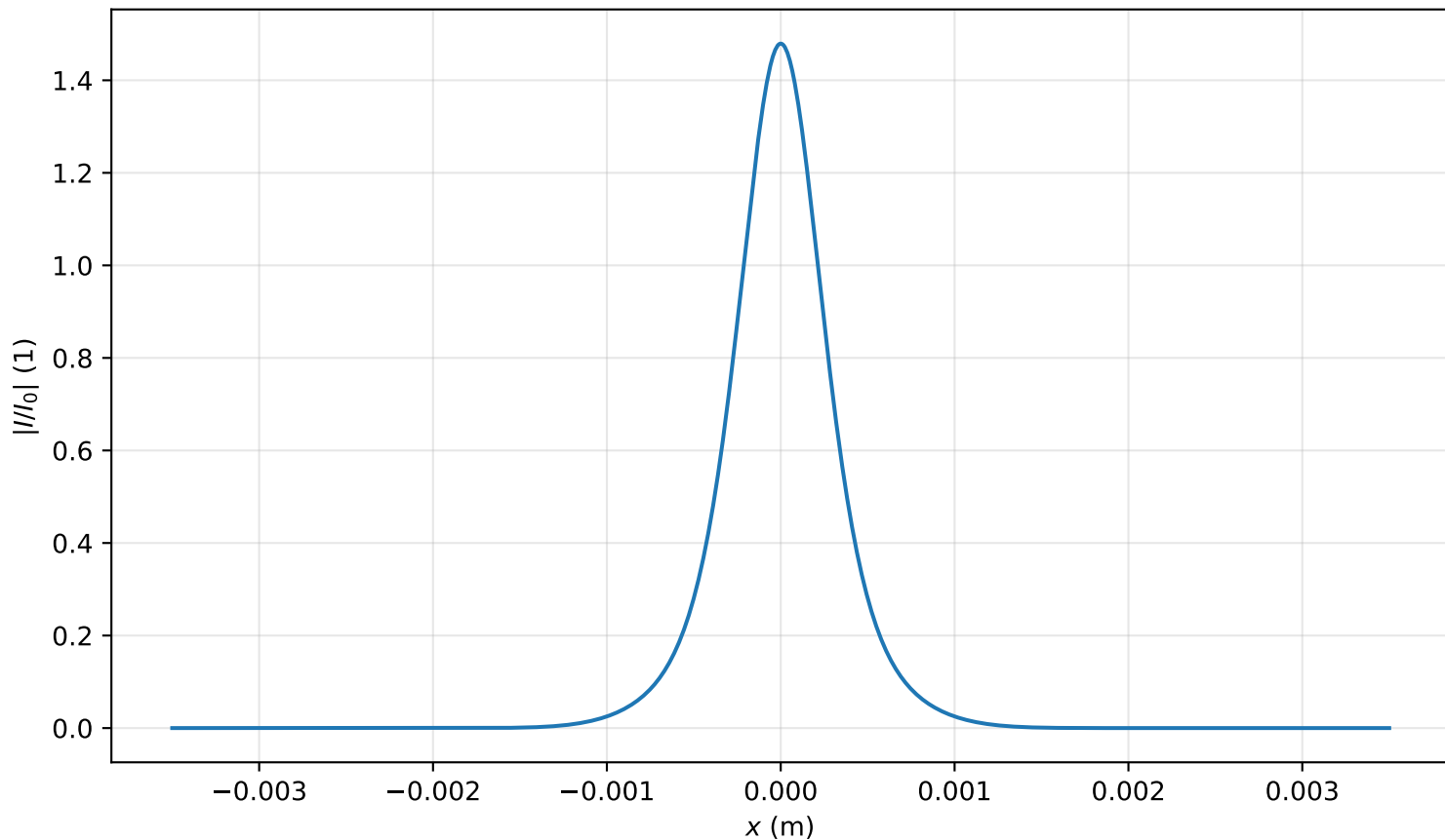
Intensity profile I(x, y = 0, z = 1.194m)/I_0 , P_{in}=0.9P_{cr} , artificial time
